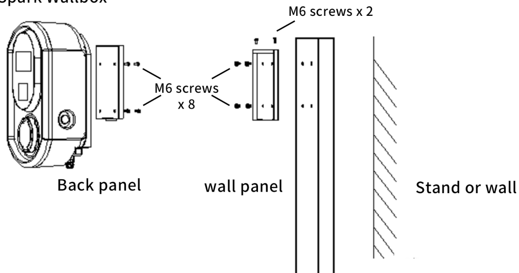
Spark Wallbox
