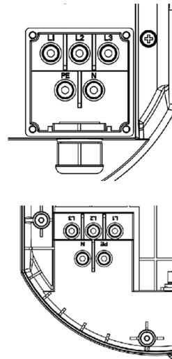
Step 2: Connect the wires of each phase according to the markings and the electrician's laws of practice, making sure that the connections are secure and mutually insulated.
