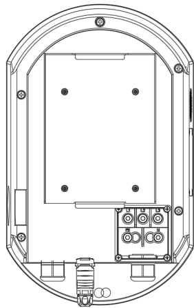
Step 1: Open the wiring window.
